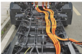
MIDDLE BUILT BATTERY PACK
